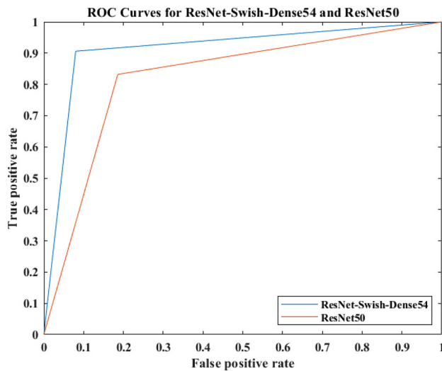
Fig. 12 AUC-ROC curves for the base and proposed models over the DFDC dataset
