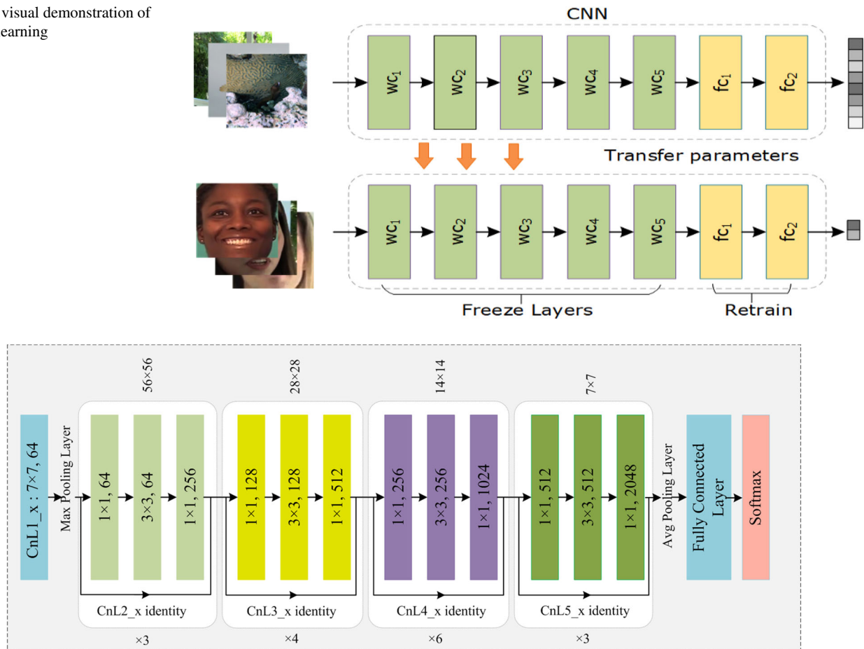
Fig. 3 The architectural description of ResNet50
