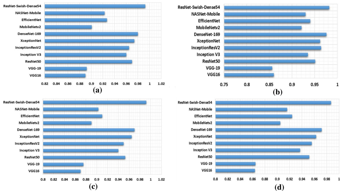
Fig. 14 Comparative analysis with the DL approaches in terms of a Accuracy, b Recall, c Precision, and d F1-score for the DFDC dataset
